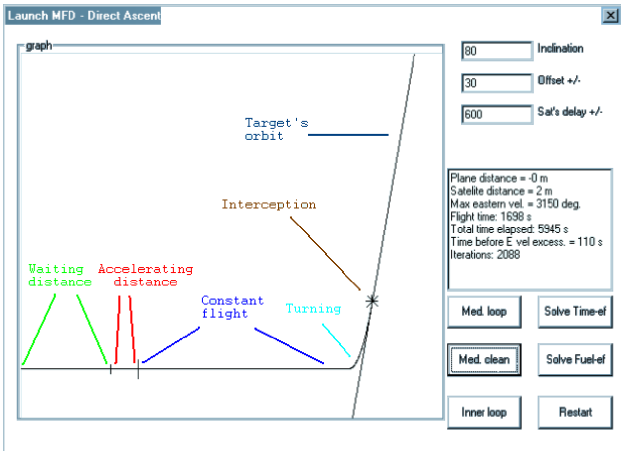
Fig. 12: Direct ascent algorithm's visual representation in Direct ascent solver (top-down view)
